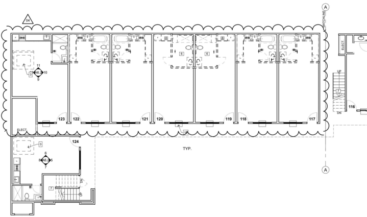
DEMO FIRST FLOOR - BUILDING 2 2 SCALE: 1/8" = 1'-0"
