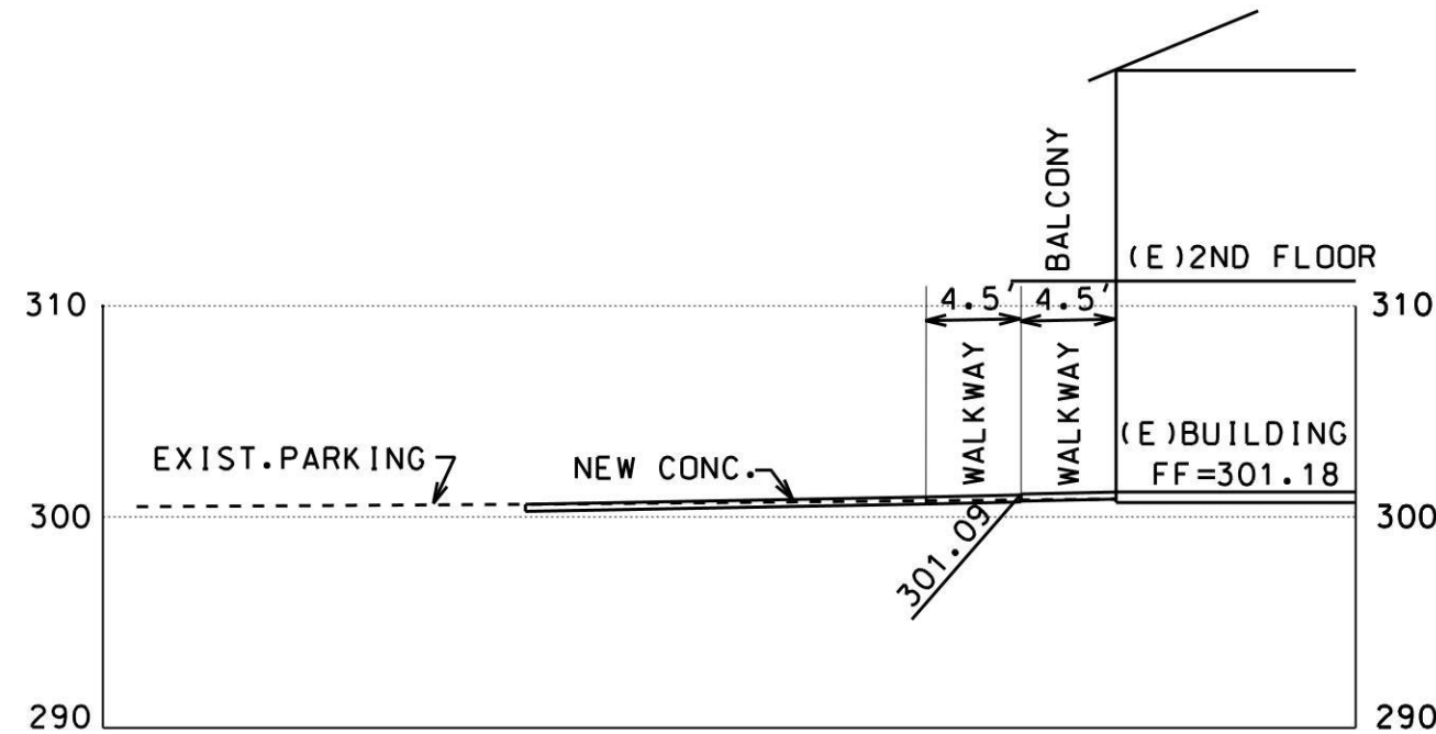
SECTION C-C
