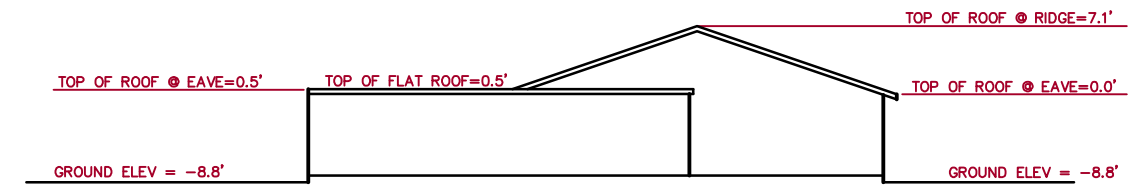
TYPICAL SECTION NTS
