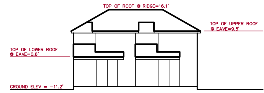
TYPICAL SECTION NTS
